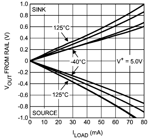
Output Voltage Swing vs. Load Current at V^+ = 5.0V
