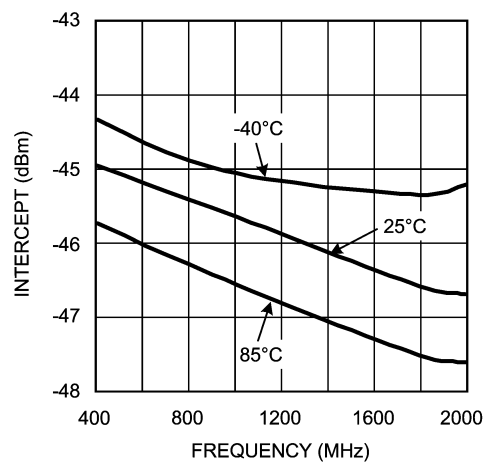
Logarithmic Intercept vs. Frequency (LMV228)
