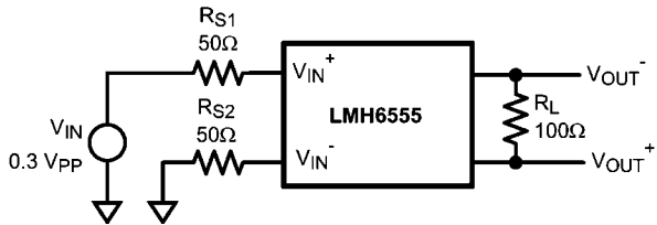
FIGURE 3. Single-Ended Input Drive
