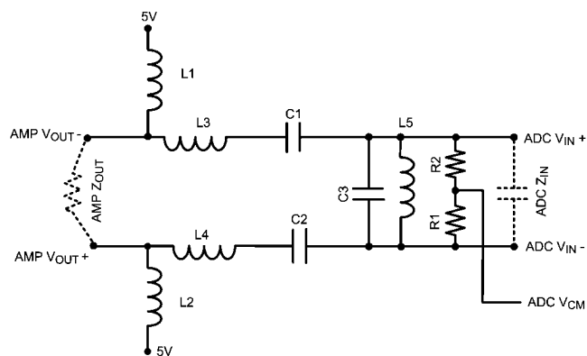
FIGURE 10. Sample Filter
