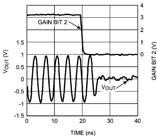
24 dB Gain Step
