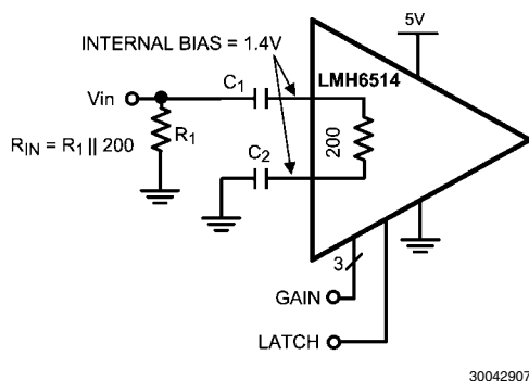
FIGURE 4. Single Ended Input (Note capacitor on grounded input)
