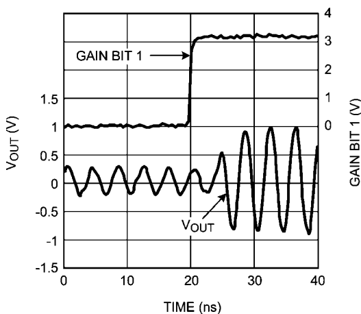
12 dB Gain Step
