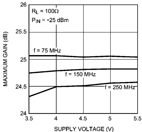
Maximum Gain vs. Supply Voltage
