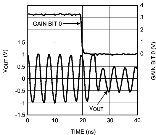
6 dB Gain Step
