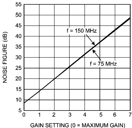
Noise Figure for All Gain Settings
