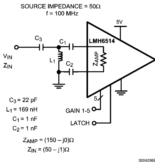
FIGURE 5. Single Ended Input with LC Matching
