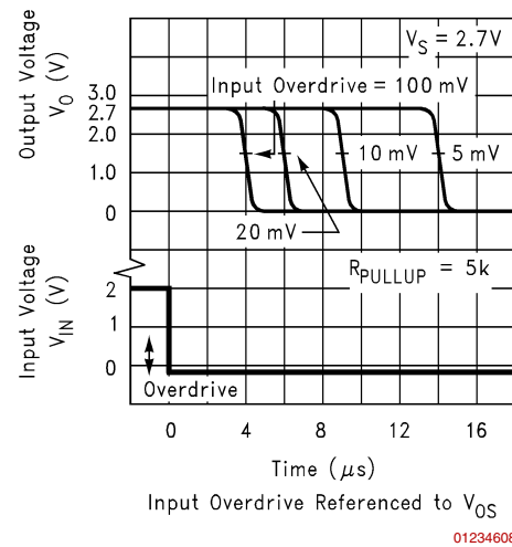
Response Time for Various Input Overdrives -t_{PHL}
