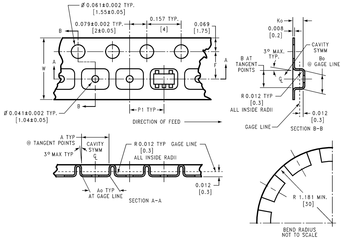
Tape Dimensions
