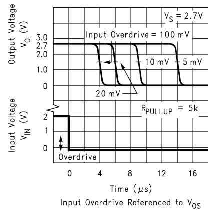
Response Time for Various Input Overdrives - t_{PHL}
