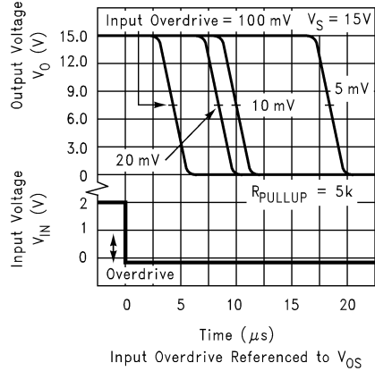
Response Time vs Various Input Overdrives – t_{PHL}
