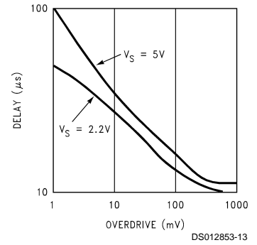
Prop Delay vs Overdrive
