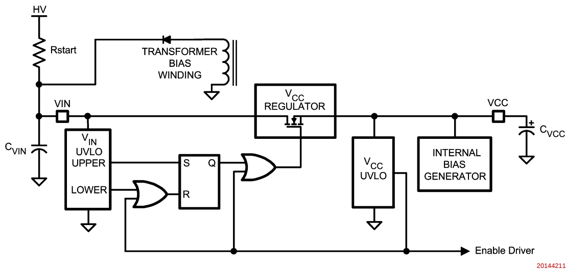
FIGURE 2. Start-Up Circuit Block Diagram
