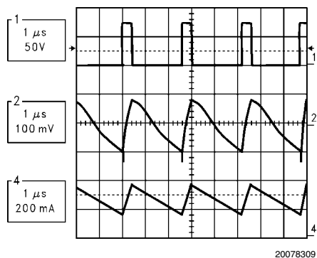
Operational Waveforms
