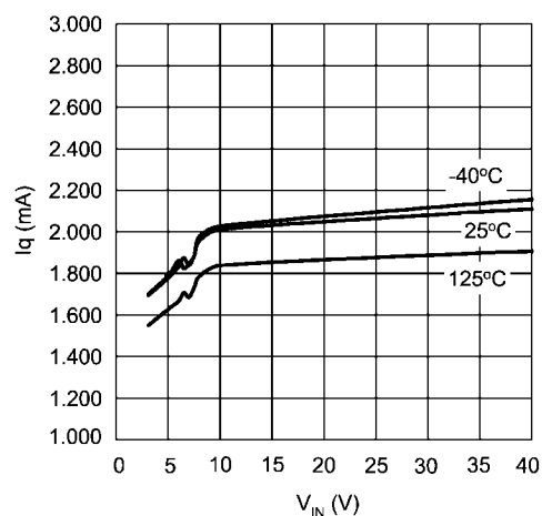
I_q (non-switching) vs V_{IN} @ f_{SW} = 700kHz
