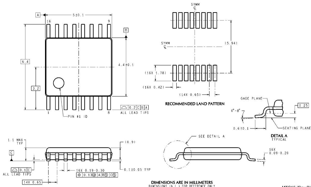
TSSOP-16 Pin Package (MTC) For Ordering, Refer to Ordering Information Table NS Package Number MTC16
