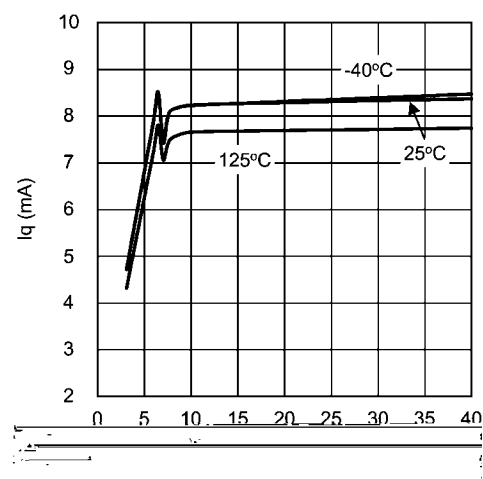
I_q (switching) vs V_{IN} @ f_{SW} = 700kHz
