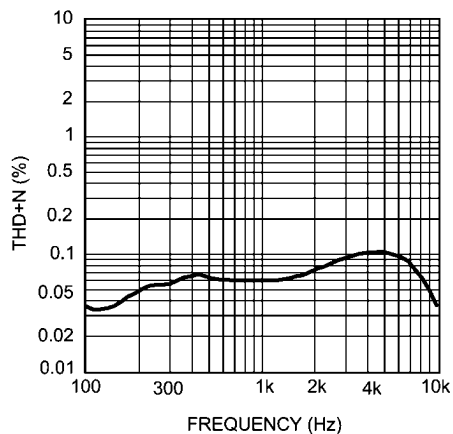
THD+N vs Frequency V_O = 4.95V_{RMS} , V_{DD} = 3.2V , Z_L = 1\mu F + 20
