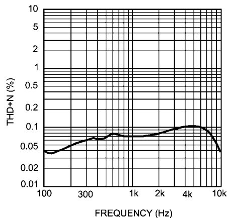
THD+N vs Frequency V_O = 4.95V_{RMS} , V_{DD} = 4.2V , Z_L = 1\mu F + 20
