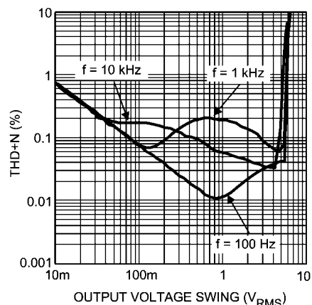
THD+N vs Output Voltage Swing V_{DD} = 3.2V , Z_L = 1\mu F + 20
