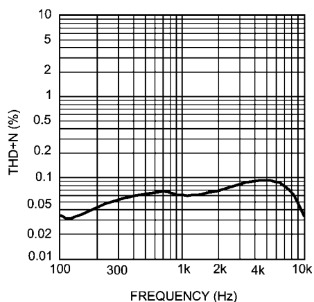
THD+N vs Frequency V_O = 4.95V_{RMS} , V_{DD} = 5V , Z_L = 1\mu F + 20
