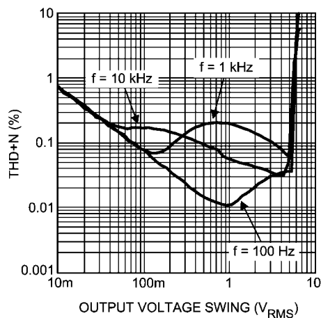
THD+N vs Output Voltage Swing V_{DD} = 5V , Z_L = 1\mu F + 20
