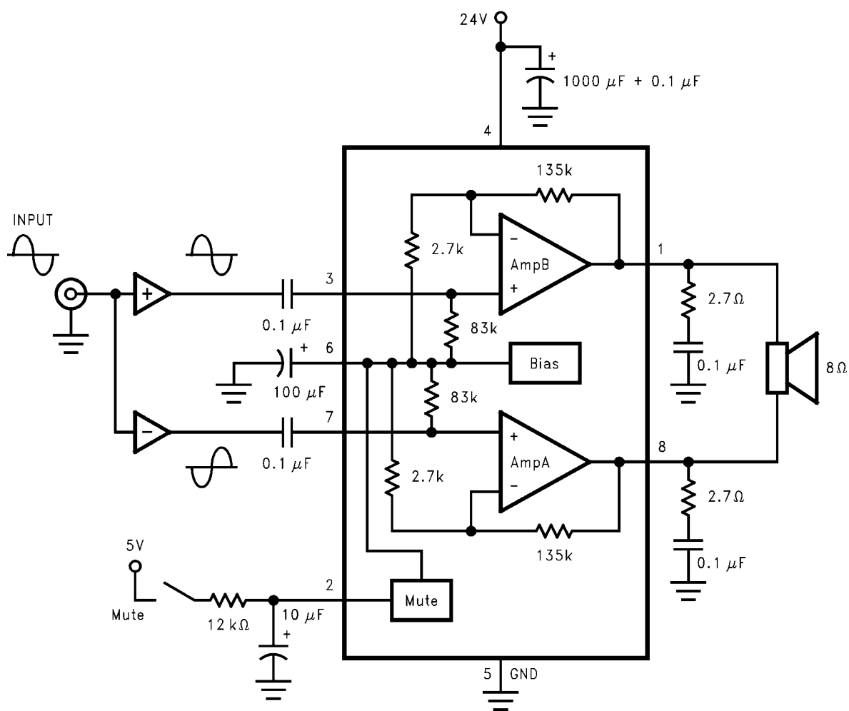
FIGURE 4. Bridge-Mode Application
