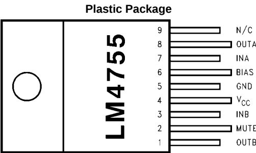
Package Description Top View Order Number LM4755T Package Number TA09A
