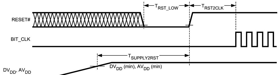
Power On Reset
