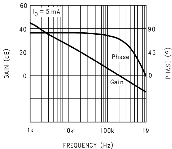
Bode Plot
