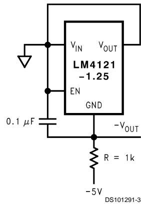
Voltage Reference with Negative Output
