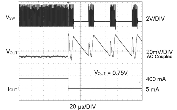
Load Transient Reponse ( V_{OUT} = 0.75V , PWM Mode to ECO Mode)
