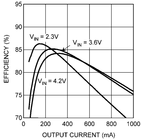
Efficiency vs. Output Current ( V_{OUT} = 0.75V , FPWM Mode)
