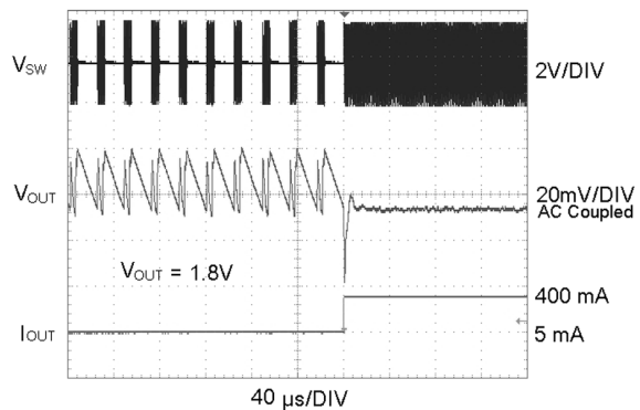
Load Transient Response ( V_{OUT} = 1.8V , ECO Mode to PWM Mode)
