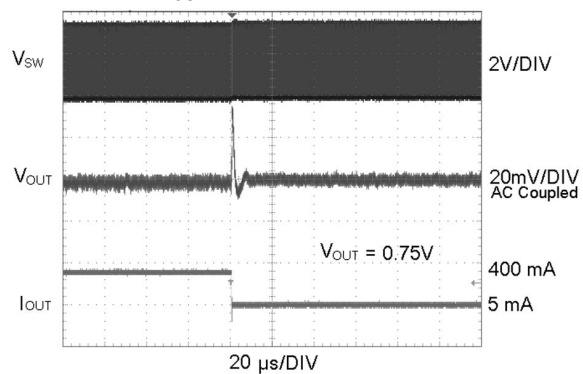
Load Transient Response ( V_{OUT} = 0.75V , FPWM Mode)
