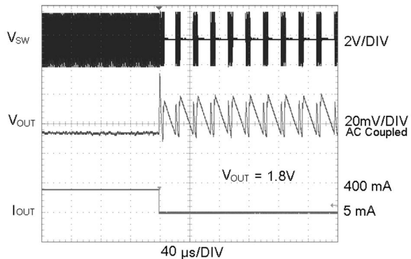
Load Transient Response ( V_{OUT} = 1.8V , PWM Mode to ECO Mode)
