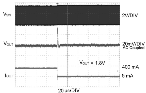
Load Transient Response ( V_{OUT} = 1.8V , FPWM Mode)
