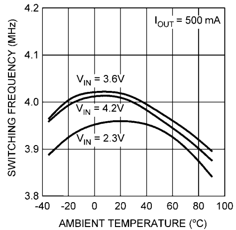
Switching Frequency vs. Temp ( V_{OUT} = 1.8V , PWM Mode)
