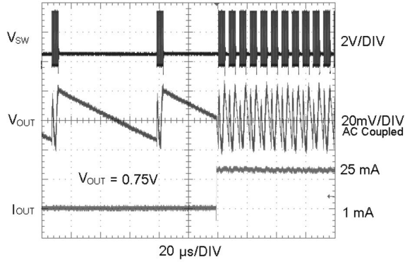
Load Transient Reponse ( V_{OUT} = 0.75V , ECO Mode 1mA to 25 mA)
