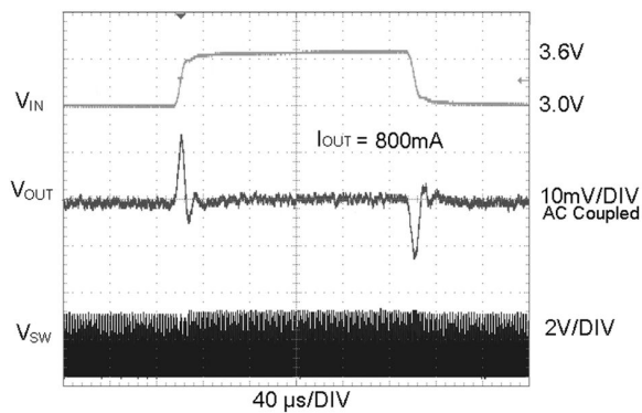
Line Transient Reponse ( V_{OUT} = 0.75V , PWM Mode)
