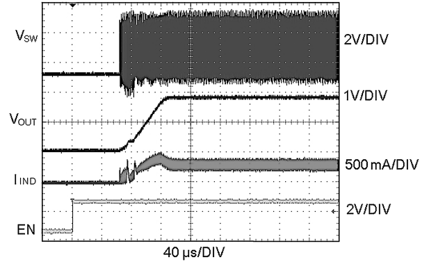
Start Up into PWM Mode ( V_{OUT} = 1.8V , R_{OUT} = 6 \Omega )
