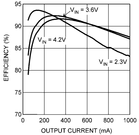
Efficiency vs. Output Current ( V_{OUT} = 1.8V , FPWM Mode)
