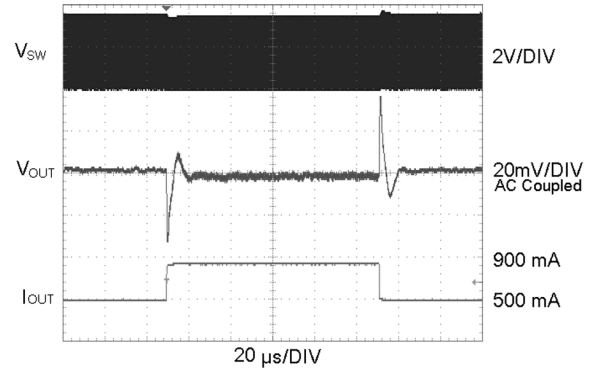
Load Transient Reponse ( V_{OUT} = 1.8V , PWM Mode)
