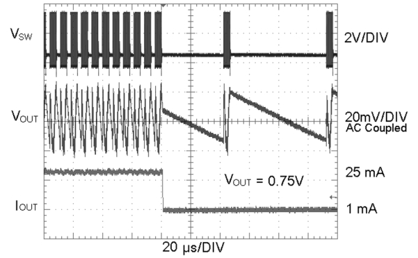
Load Transient Reponse ( V_{OUT} = 0.75V , ECO Mode 25 mA to 1mA)
