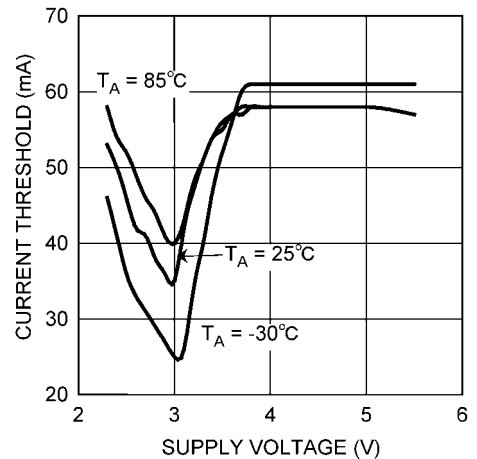
Load Current Threshold vs. Supply Voltage ( V_{OUT} = 1.8V , ECO Mode to PWM Mode)
