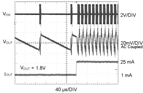
Load Transient Reponse ( V_{OUT} = 1.8V , ECO Mode 1mA to 25 mA)
