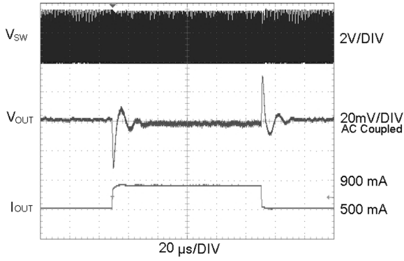
Load Transient Reponse ( V_{OUT} = 0.75V , PWM Mode)
