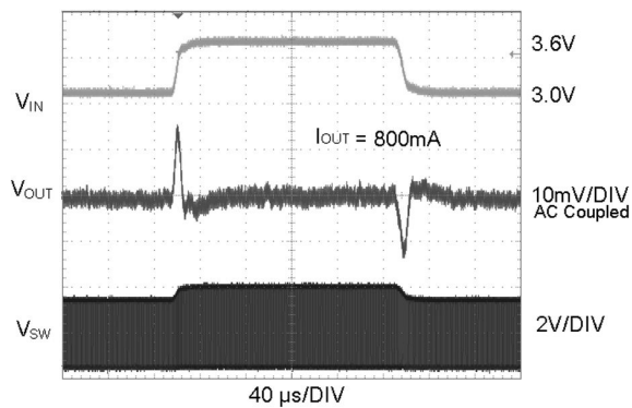
Line Transient Reponse ( V_{OUT} = 1.8V , PWM Mode)
