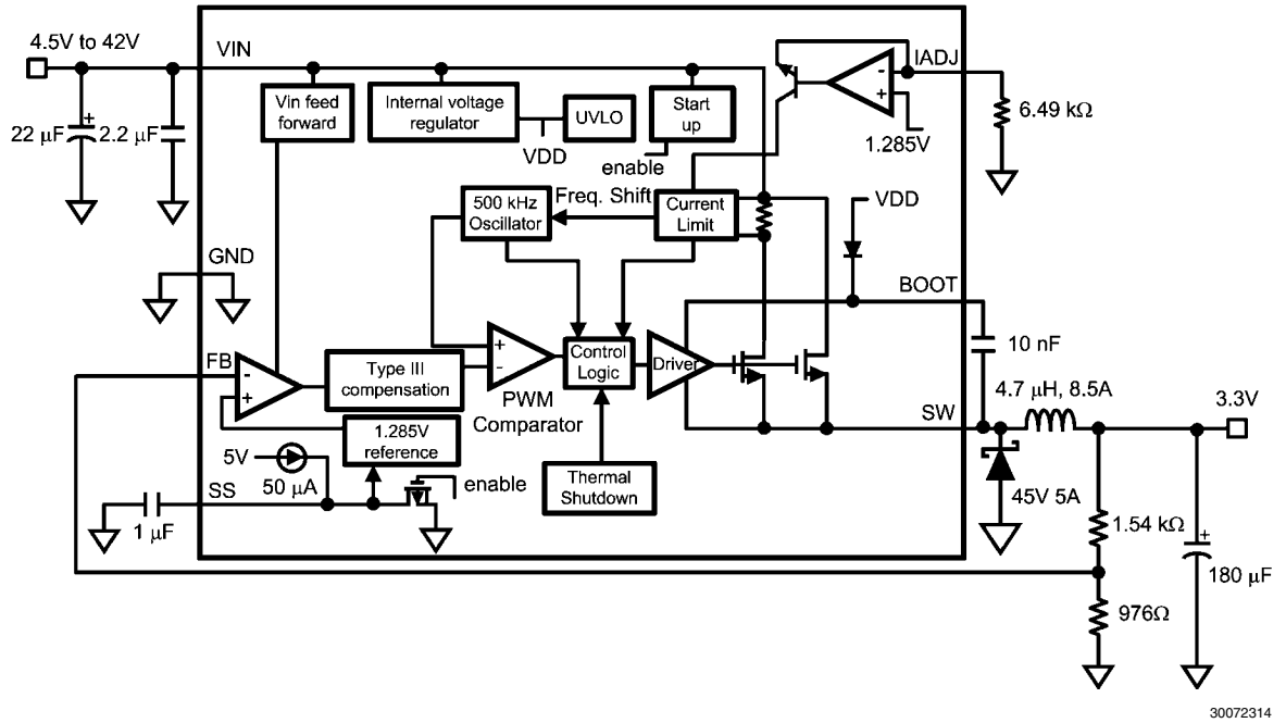
FIGURE 1. 3.3V V_{\text{OUT}} at 4.5A
