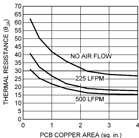
FIGURE 12. Thermal Resistance vs PCB Area (4 Layer Board)
