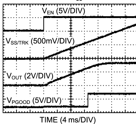
Startup with C_{SS} = 100 nF
