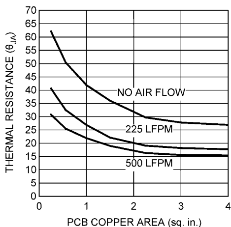
FIGURE 10. Thermal Resistance vs PCB Area (4 Layer Board)
