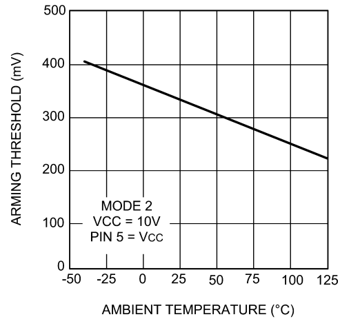
Mode 2 Minimum Arming Threshold vs Temperature
