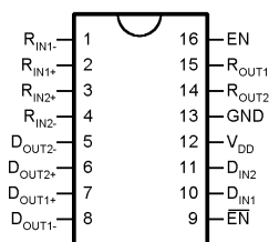
Dual-In-Line
