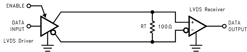
FIGURE 10. Point-to-Point Application
