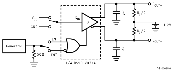
FIGURE 4. Driver TRI-STATE Delay Test Circuit
