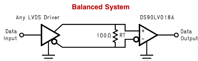
FIGURE 3. Point-to-Point Application
