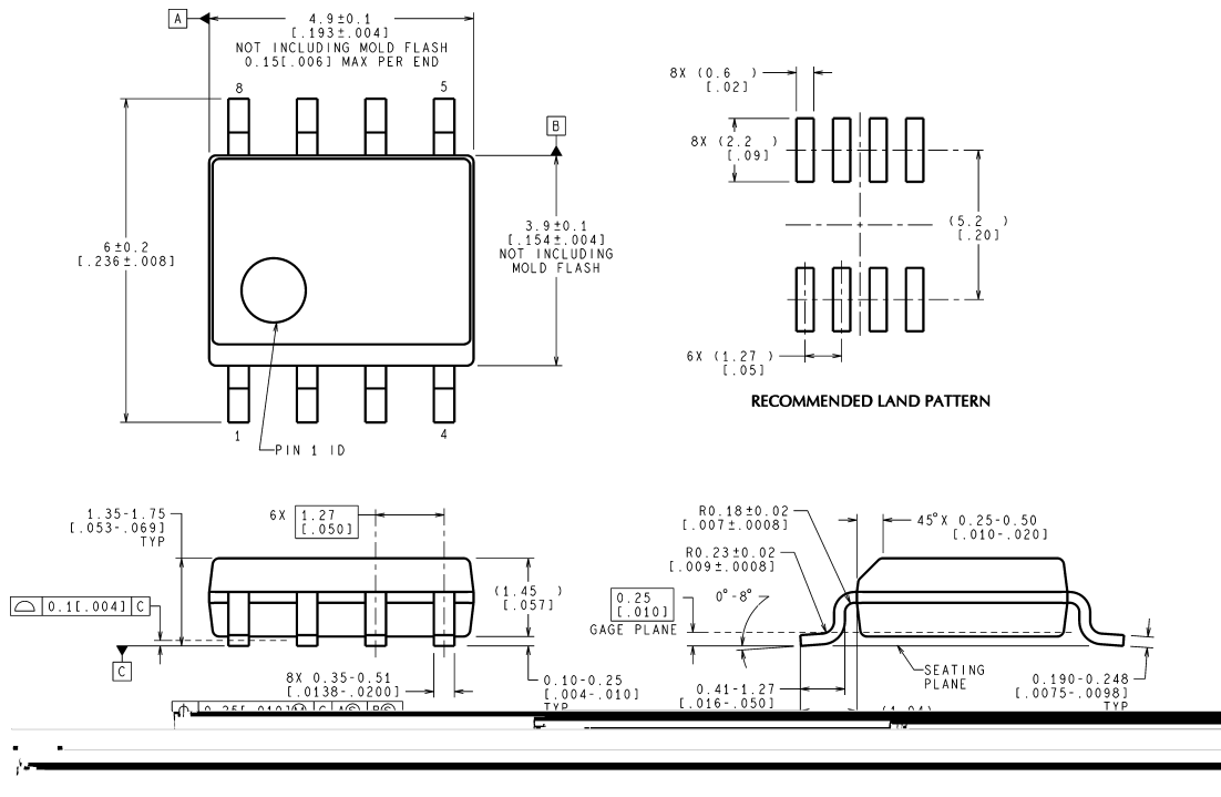
8-Lead (0.150" Wide) Molded Small Outline Package, JEDEC Order Number DS90LV018ATM NS Package Number M08A
