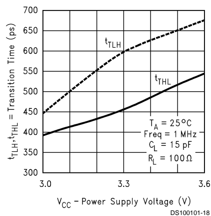
Transition Time vs Power Supply Voltage
