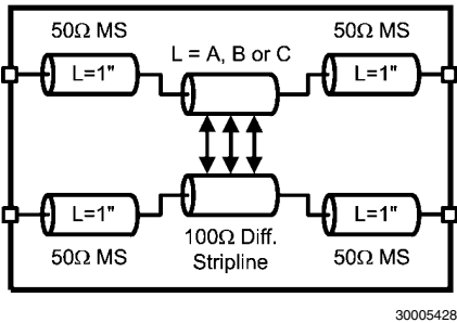
FIGURE 6. Test Channel Description
