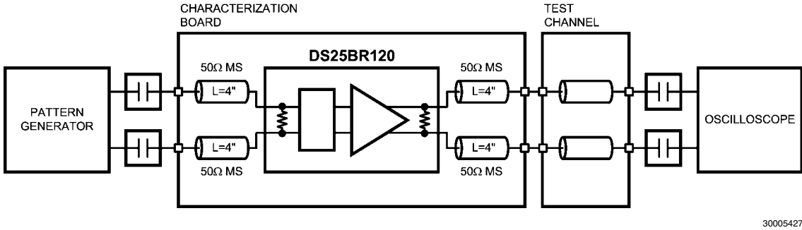
FIGURE 5. Pre-emphasis Performance Test Circuit
