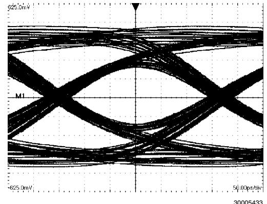
An Equalized (with PE) 3.125 Gbps NRZ PRBS-7 After 40" Differential FR-4 Stripline V:125 mV / DIV, H:50 ps / DIV
