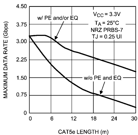
30005338 Maximum Data Rate as a Function of CAT5e (Belden 1700A) Length DS25BR120 Used as a Driver DS25BR110 Used as a Receiver
