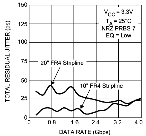
Total Jitter as a Function of Data Rate
