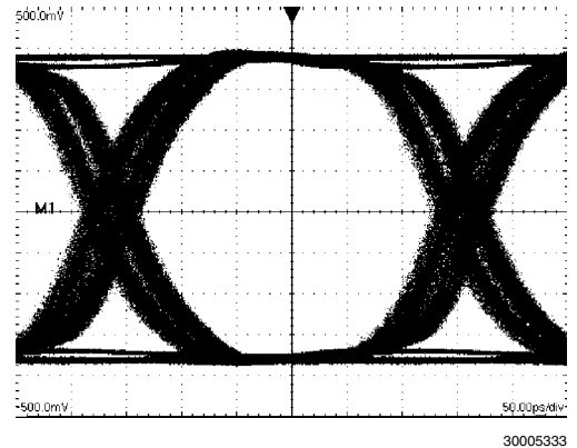
An Equalized 3.125 Gbps NRZ PRBS-7 After 70" Differential FR-4 Stripline V:100 mV / DIV, H:50 ps / DIV
