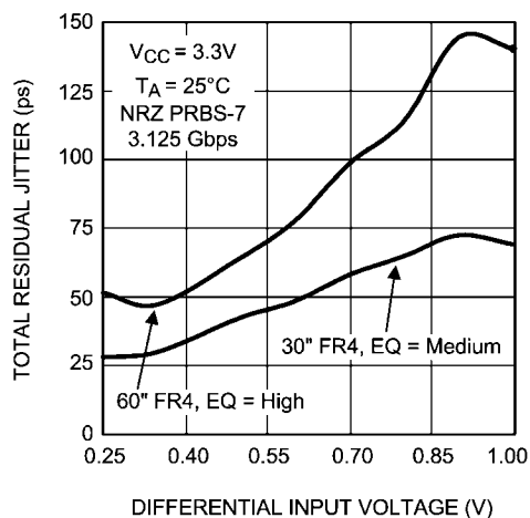
30005347 Total Jitter as a Function of Input Amplitude
