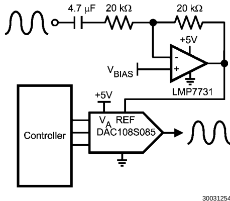
FIGURE 16. Programmable Attenuator
