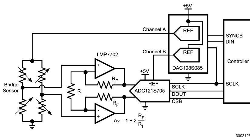
FIGURE 15. Driving an ADC Reference
