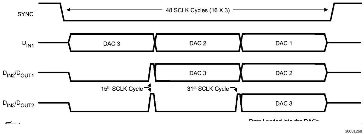
FIGURE 7. Daisy Chain Timing Diagram
