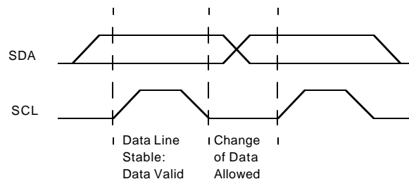
Figure 39. Bit Transfer
