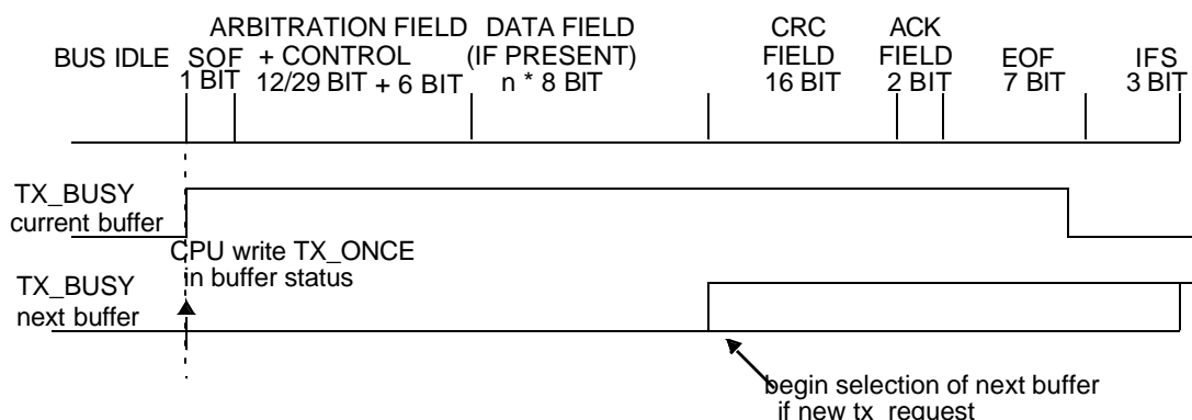
Figure 64. Data Transmission
