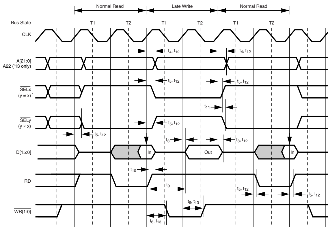
Figure 80. Late Write Between Normal Read Cycles (No Wait States)
