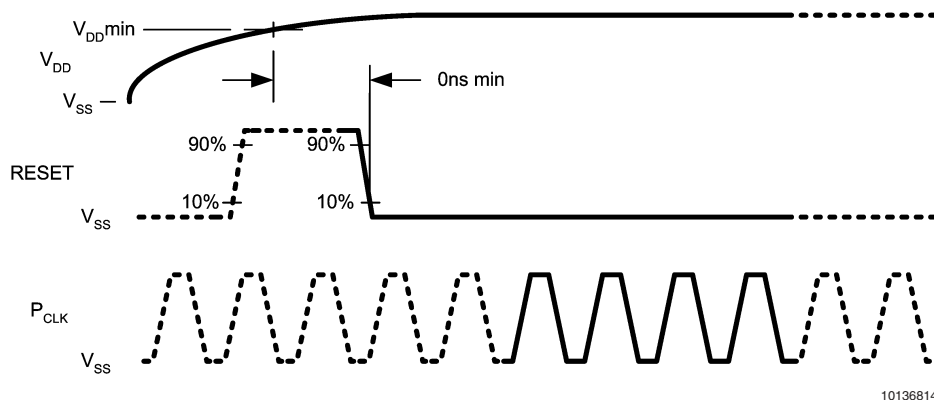
FIGURE 5. Power-On Reset Sequence with Manual Reset
