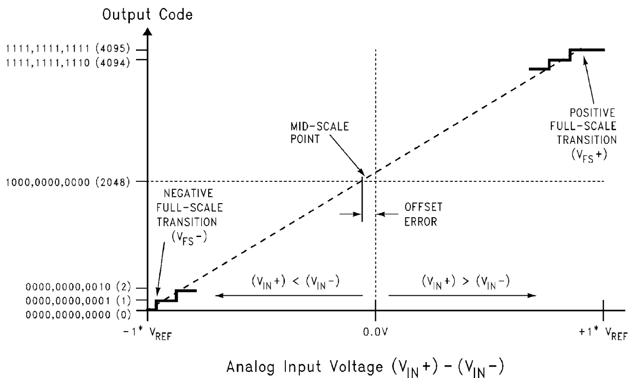
FIGURE 4. Transfer Characteristic
