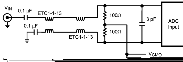
FIGURE 8. High Input Frequency Transformer Drive Circuit
