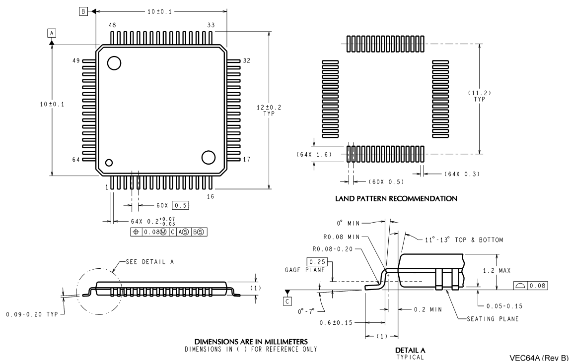
64-Lead TQFP Package Ordering Number ADC12DL066CIVS NS Package Number VEEC64A
