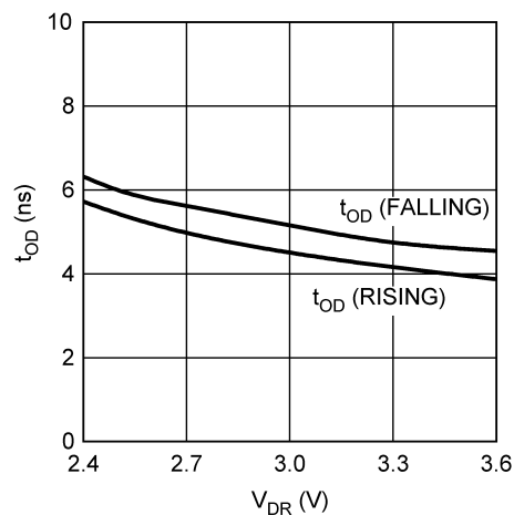
t_{OD} vs. V_{DR} , V_A = V_D = 3.6V Parallel Output Mode
