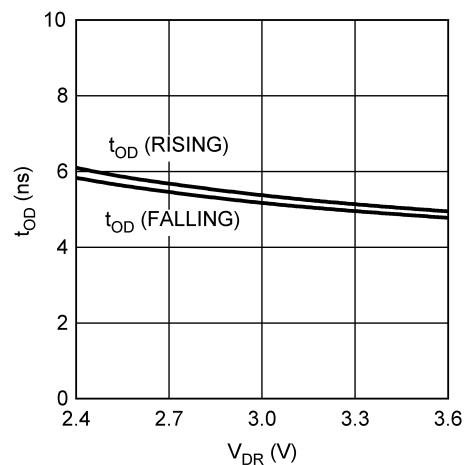
t_{OD} vs. V_{DR} , V_A = V_D = 3.6V Multiplex Output Mode
