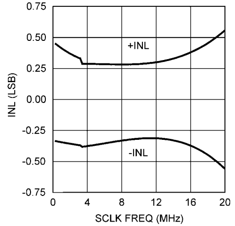
INL vs. SCLK FREQUENCY
