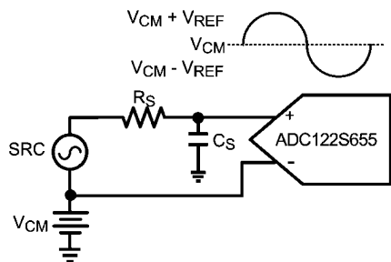
FIGURE 8. Single-Ended Input
