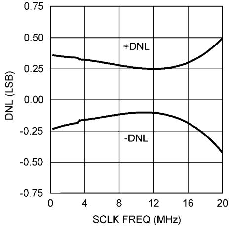
DNL vs. SCLK FREQUENCY
