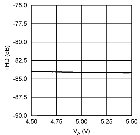
THD vs. V_A
