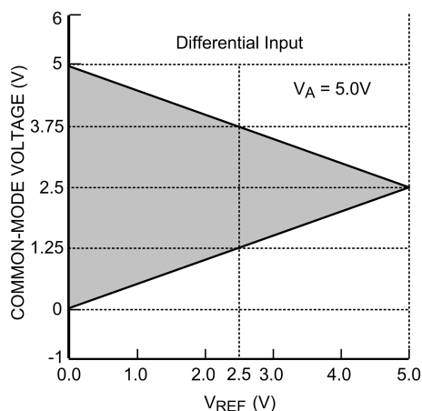
FIGURE 9. V_{CM} range for Differential Input operation
