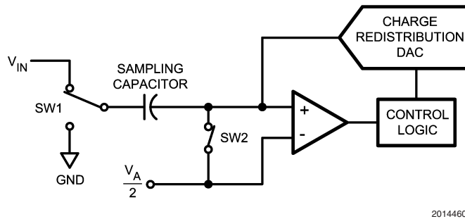
FIGURE 3. ADC121S051 in Track Mode
