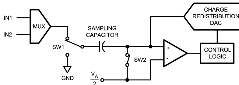
FIGURE 1. ADC102S021 in Track Mode
