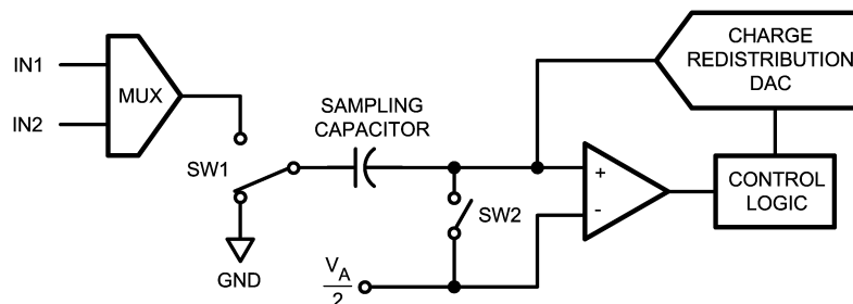
FIGURE 2. ADC102S021 in Hold Mode
