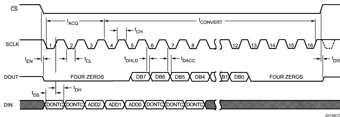
FIGURE 2. ADC088S022 Serial Timing Diagram
