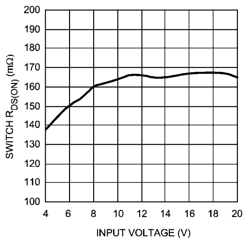
Adjustable Buck R_{DS(ON)} vs. Input Voltage
