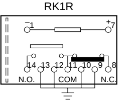
R type contact arrangement
