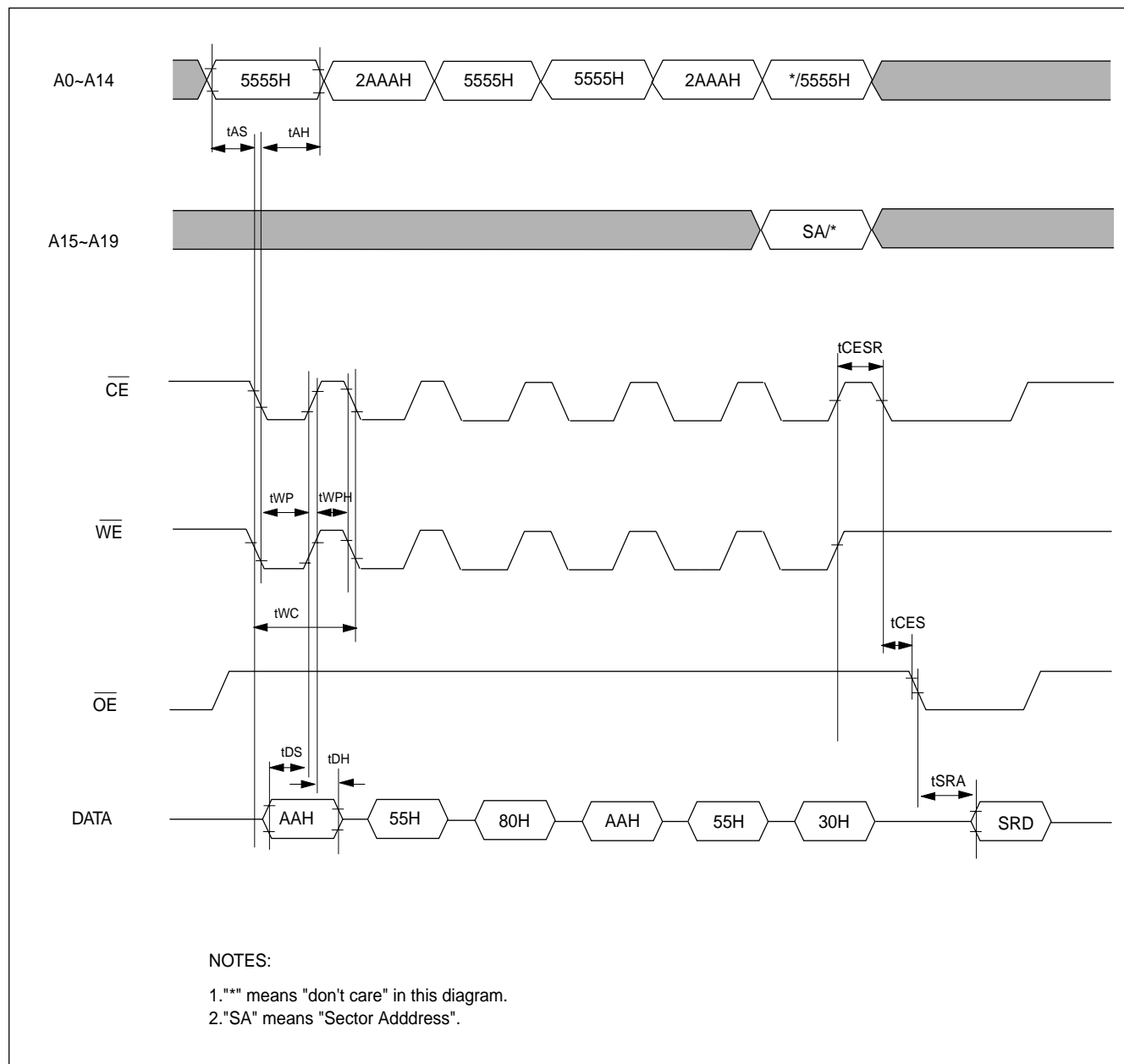
Figure 9. AUTOMATIC SECTOR/CHIP ERASE TIMING WAVEFORMS
