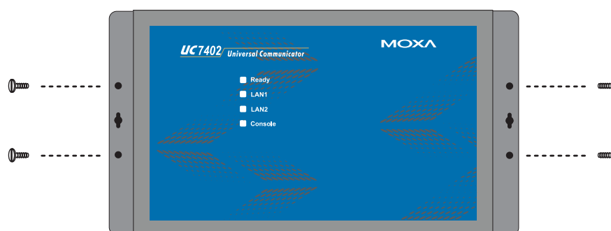
Figure B: UC-7402 Universal Communicator—Wall Mounting Brackets (top view)
