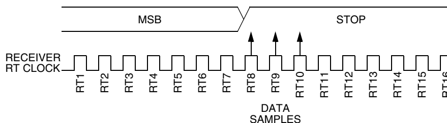
Figure 14-10. Slow Data
