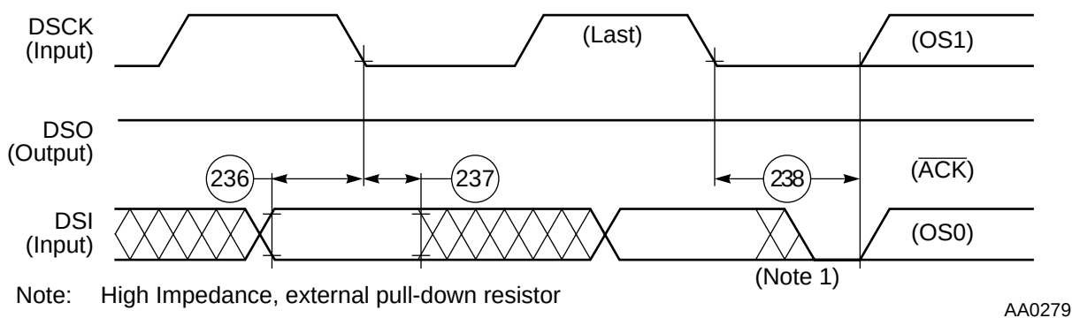
Figure 4-24. DSP56012 OnCE Data I/O to Status Timing
