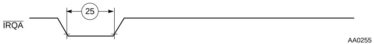
Figure 4-6. Recovery from Stop State Using \overline{\text{IRQA}}
