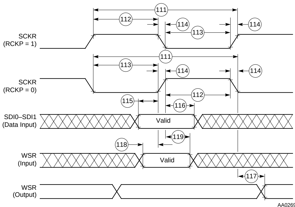
Figure 4-13. SAI Receiver Timing
