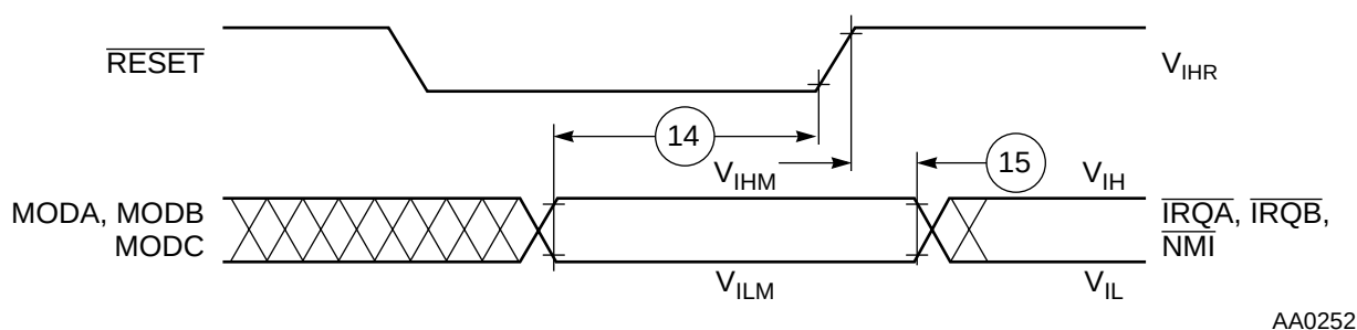
Figure 4-3. Operating Mode Select Timing
