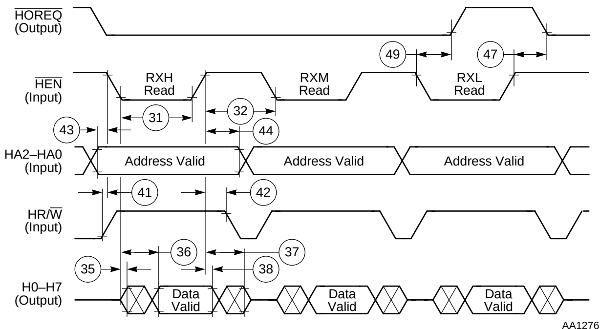
Figure 4-9. Host Read Cycle (Non-DMA Mode)
