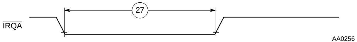
Figure 4-7. Recovery from Stop State Using \overline{\text{IRQA}} Interrupt Service
