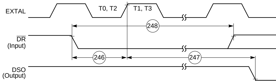
Figure 4-29. Synchronous Recovery from Wait State
