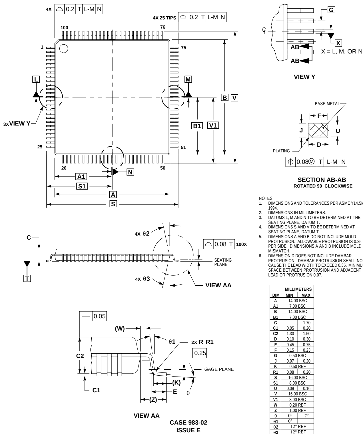
Figure 5-3. 100-Pin Thin Quad Flat Pack (TQFP) Mechanical Information
