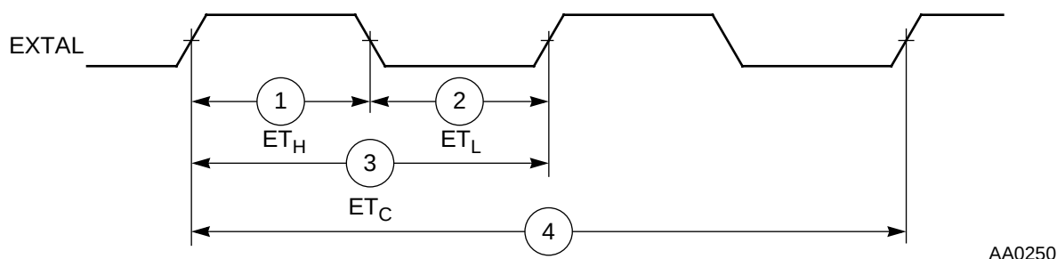
Figure 4-1. External Clock Timing
