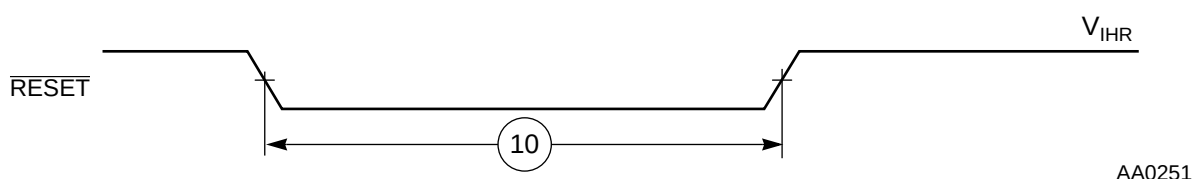
Figure 4-2. Reset Timing
