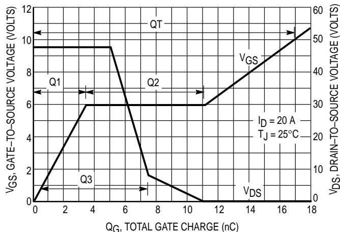
Figure 7. Gate-To-Source and Drain-To-Source Voltage versus Total Charge
