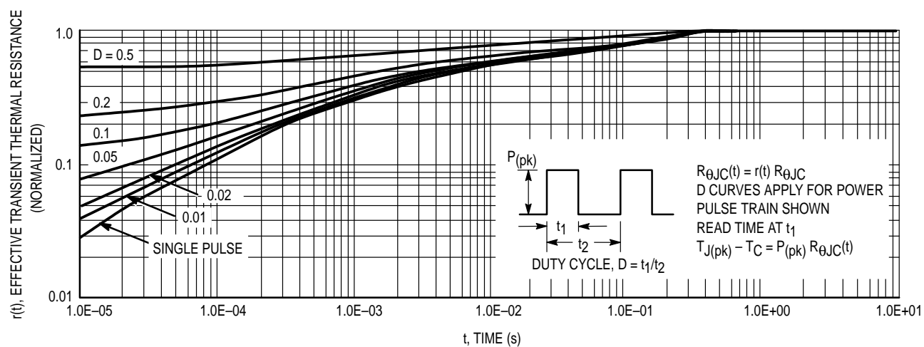
Figure 13. Thermal Response
