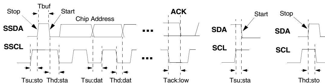
Figure 11. SSDA/SSCL Timing
