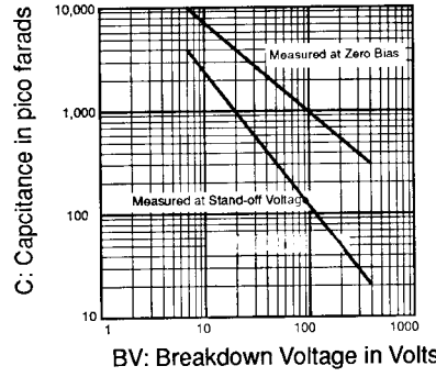
FIGURE 2 TYPICAL CAPACITANCE VS. BREAKDOWN VOLTAGE
