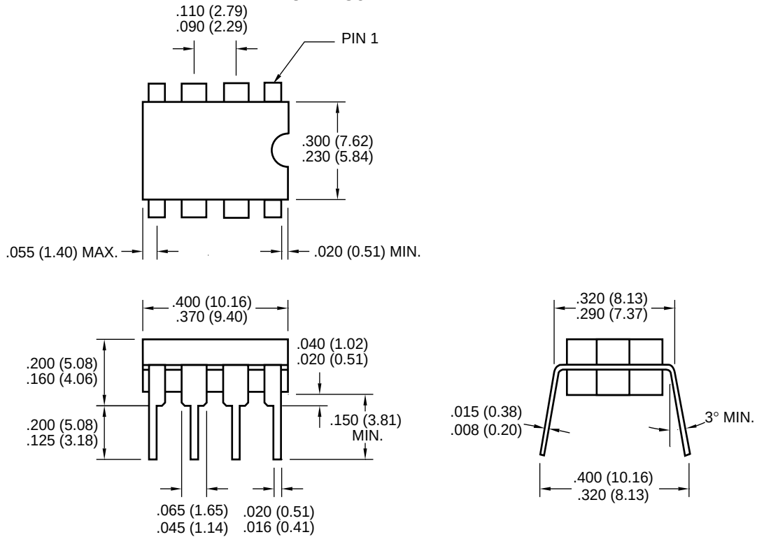
8-Pin Plastic DIP
