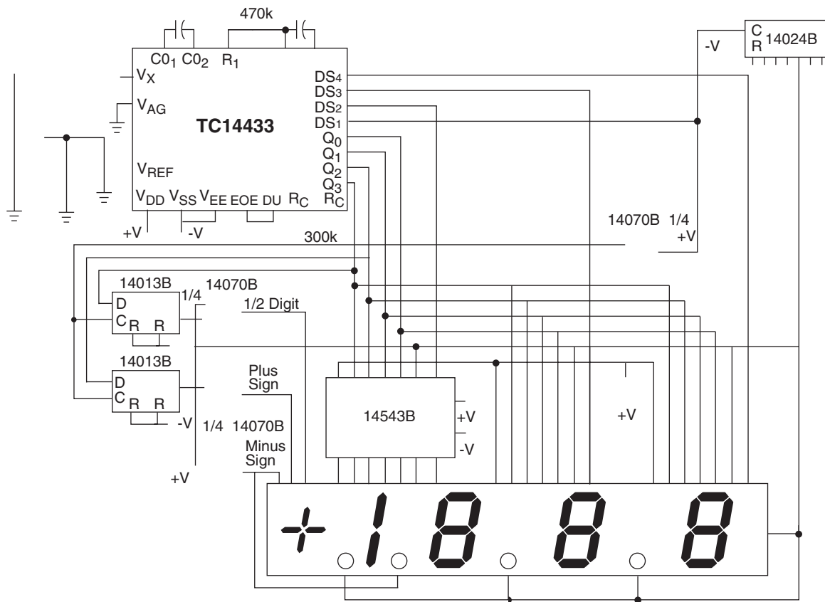
FIGURE 4-1: 3-1/2 DIGIT VOLTMETER WITH LCD DISPLAY
