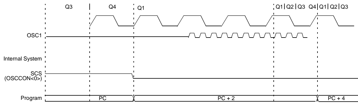
FIGURE 2-10: TIMING FOR TRANSITION BETWEEN TIMER1 AND OSC1 (RC, EC)
