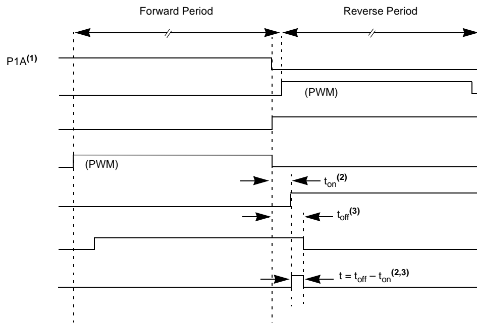
FIGURE 16-8: PWM DIRECTION CHANGE AT NEAR 100% DUTY CYCLE
