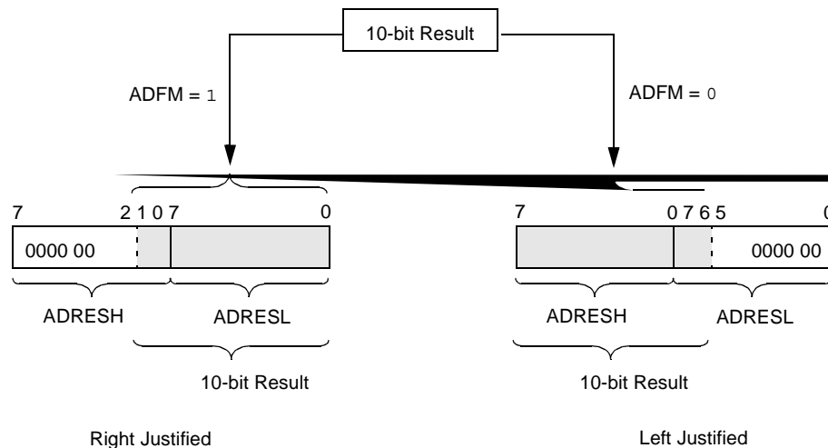
FIGURE 20-3: A/D RESULT JUSTIFICATION
