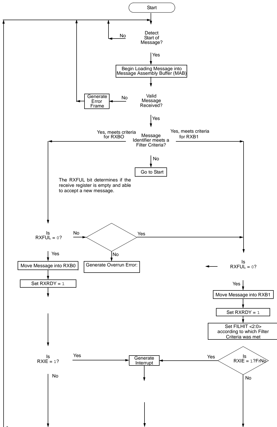
FIGURE 19-5: INTERNAL MESSAGE RECEPTION FLOWCHART
