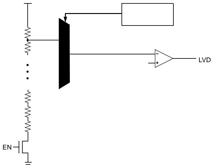
FIGURE 23-3: LOW-VOLTAGE DETECT (LVD) WITH EXTERNAL INPUT BLOCK DIAGRAM
