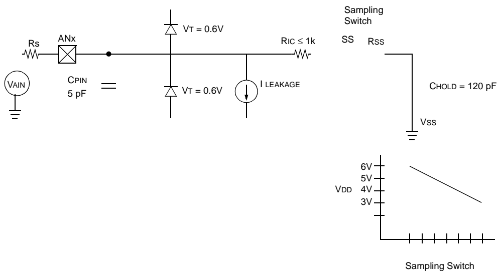
FIGURE 20-2: ANALOG INPUT MODEL
