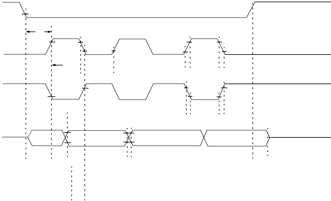
FIGURE 27-15: EXAMPLE SPI™ SLAVE MODE TIMING (CKE = 0)
