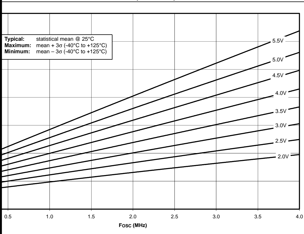
TYPICAL I_{DD} vs. F_{osc} OVER V_{DD} (XT MODE)
