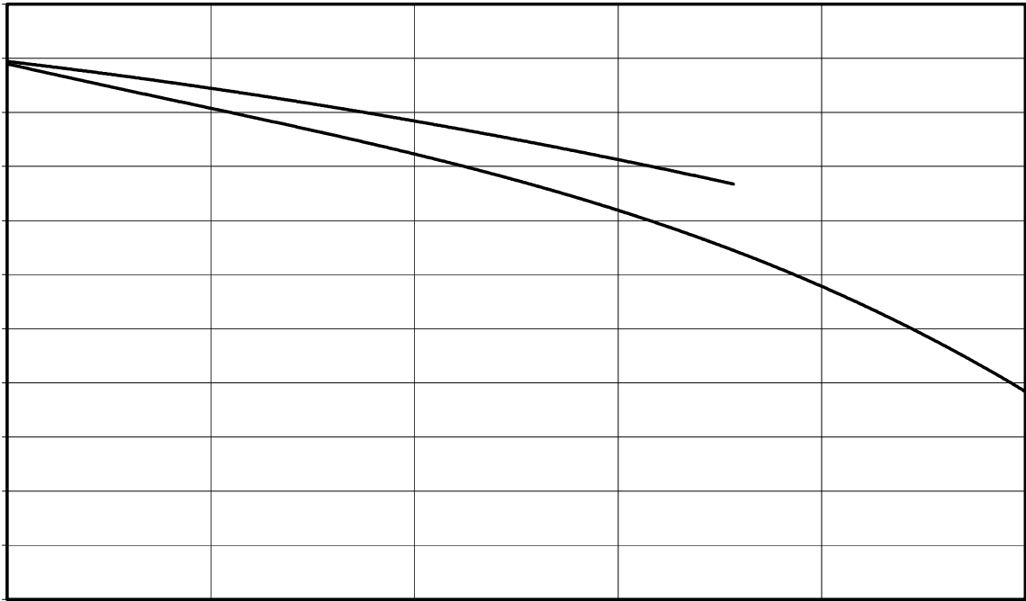
FIGURE 28-21: TYPICAL, MINIMUM AND MAXIMUM V_{OH} vs. I_{OH} ( V_{DD} = 5V , -40^{\circ}C TO +125^{\circ}C )
