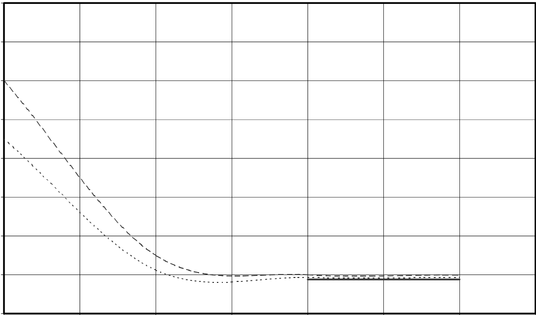
FIGURE 28-28: A/D NONLINEARITY vs. V_{REFH} ( V_{DD} = V_{REFH} , -40^{\circ}C TO +125^{\circ}C )
