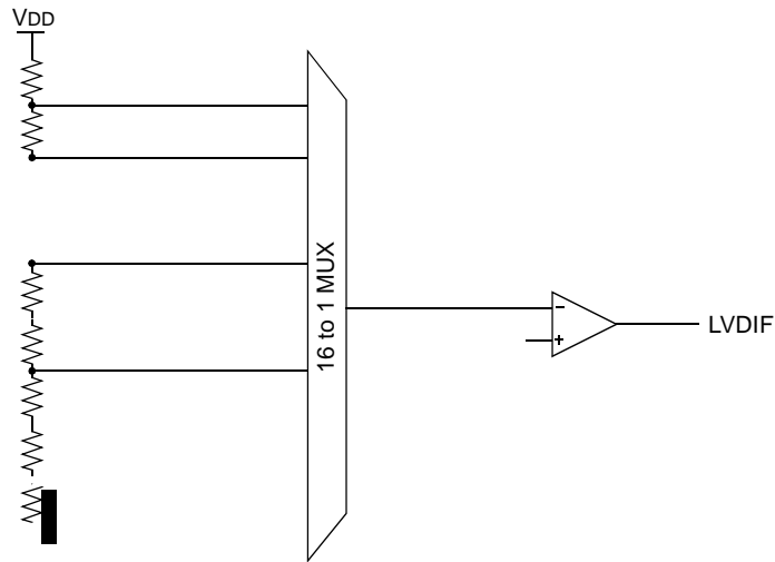
FIGURE 23-2: LOW-VOLTAGE DETECT (LVD) BLOCK DIAGRAM
