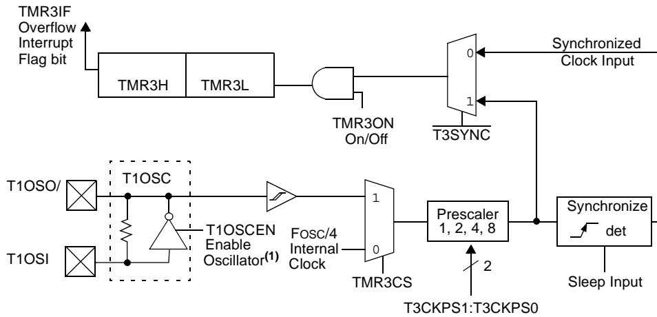
FIGURE 14-1: TIMER3 BLOCK DIAGRAM
