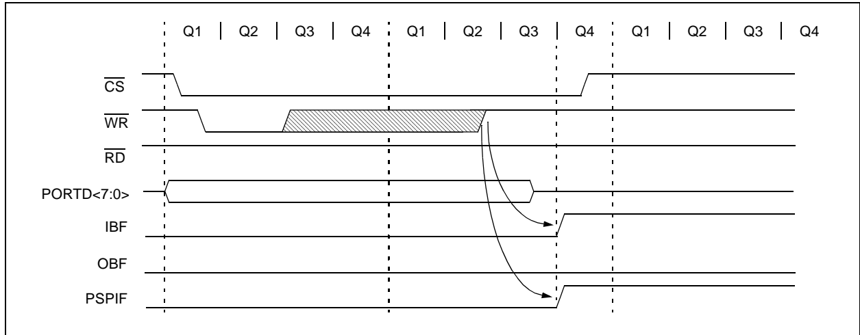
FIGURE 10-25: PARALLEL SLAVE PORT WRITE WAVEFORMS
