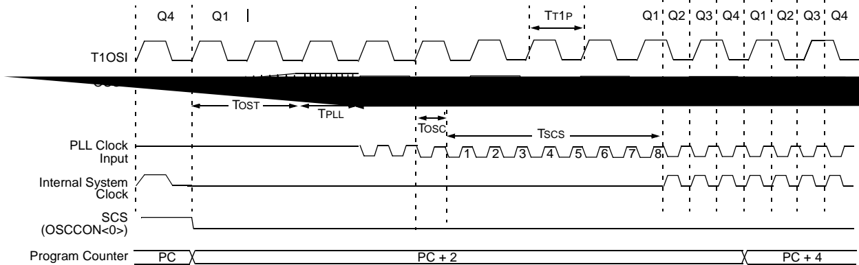
FIGURE 2-10: TIMING FOR TRANSITION BETWEEN TIMER1 AND OSC1 (HS WITH PLL ACTIVE, SCS1 = 1)
