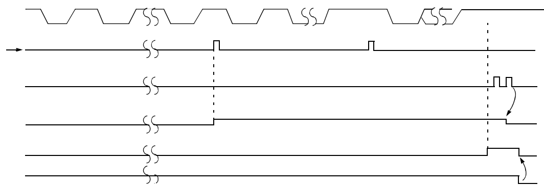
FIGURE 17-7: ASYNCHRONOUS RECEPTION
