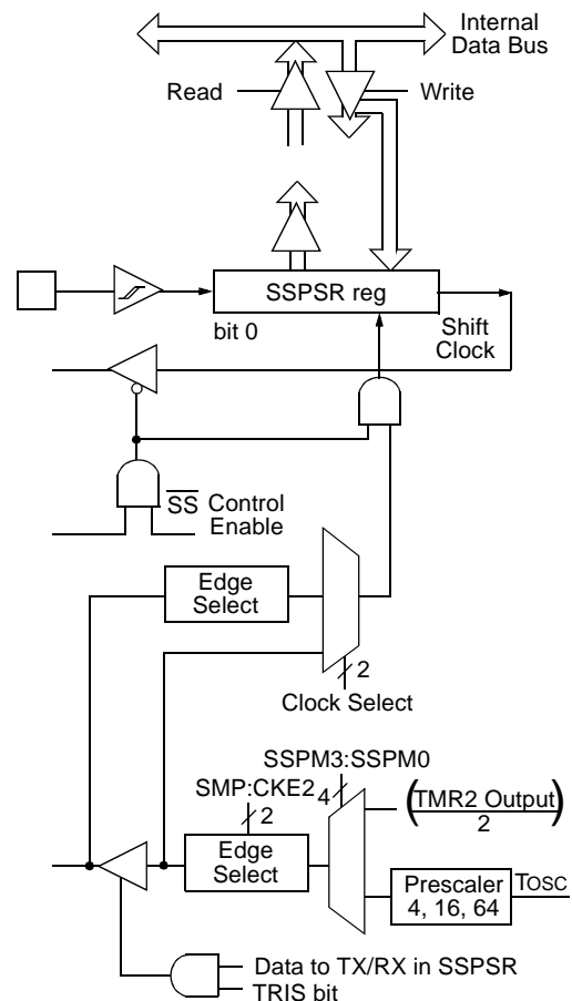
FIGURE 16-1: MSSP BLOCK DIAGRAM (SPI™ MODE)
