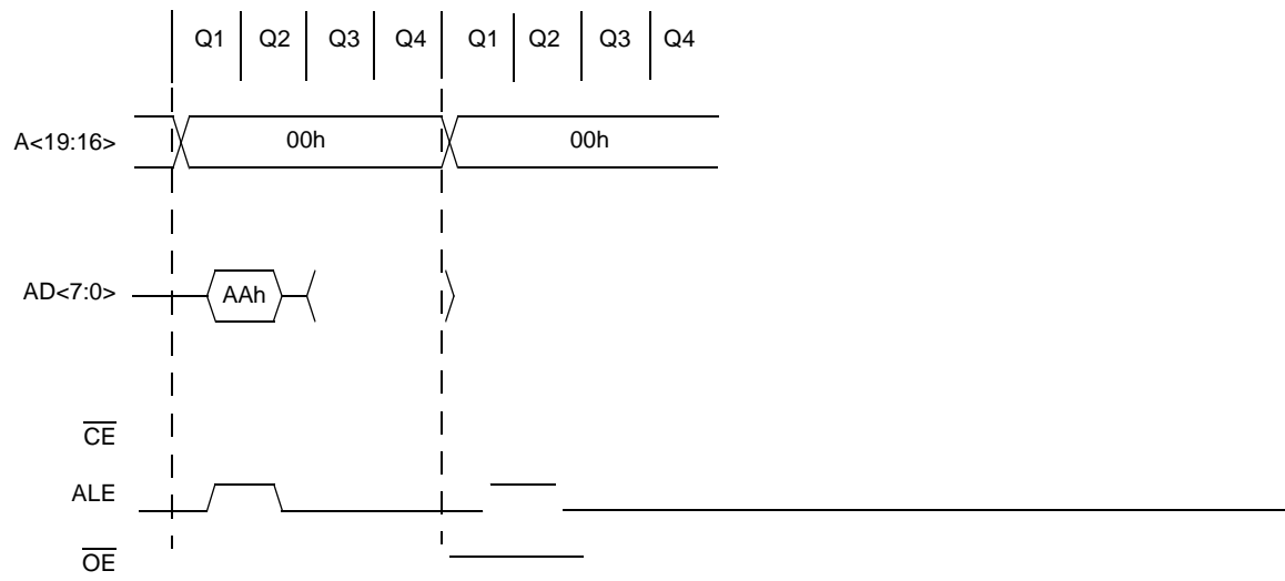
FIGURE 7-10: EXTERNAL MEMORY BUS TIMING FOR SLEEP (MICROPROCESSOR MODE)
