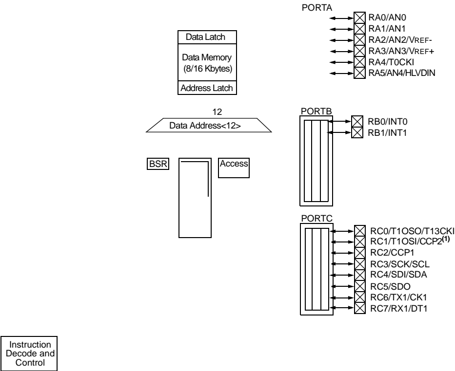
FIGURE 1-1: PIC18F6310/6410 (64-PIN) BLOCK DIAGRAM
