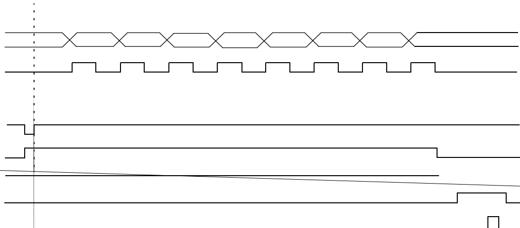
FIGURE 17-13: SYNCHRONOUS RECEPTION (MASTER MODE, SREN)
